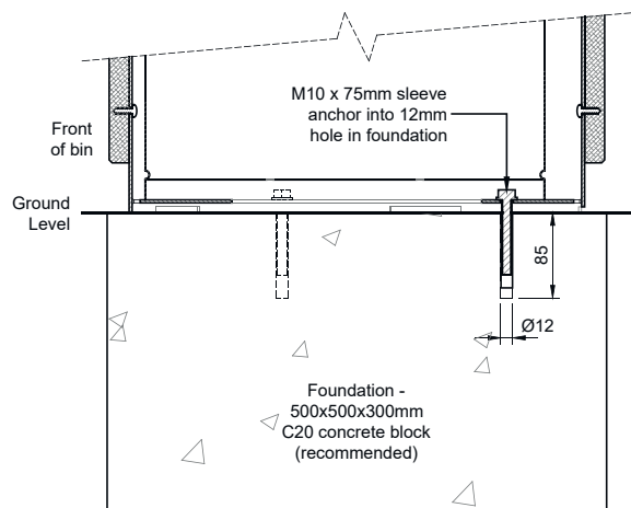
Fixing detail
