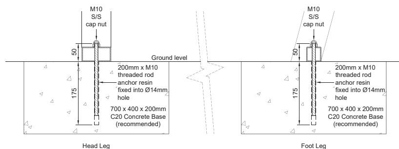
Leg Fixing Details
