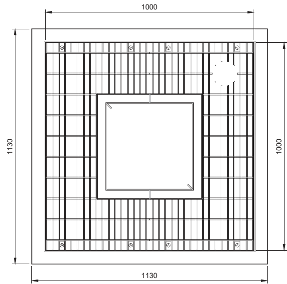
Skop tree guard set out
