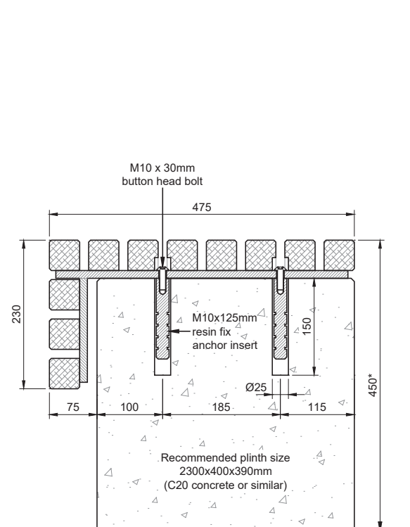
Bench base fix detail
