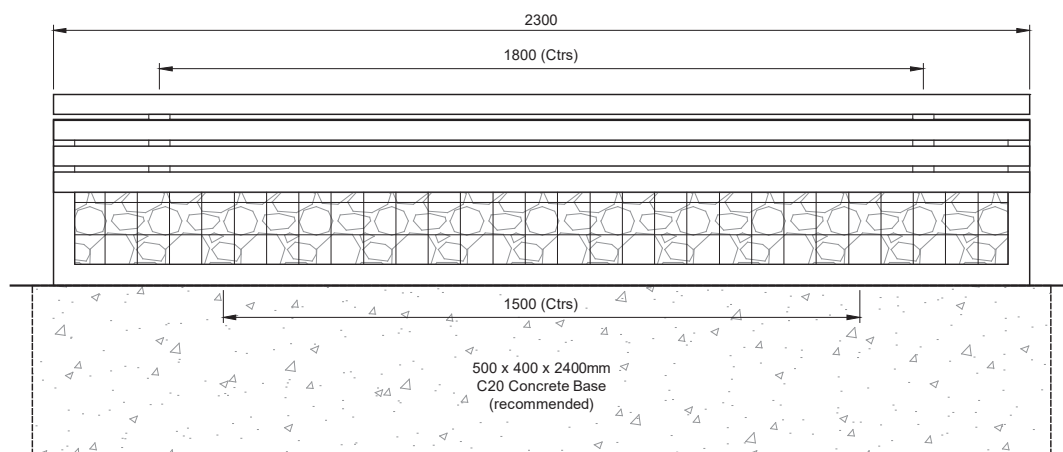
Tord Gabion Bench (same fixing centres for seat)
