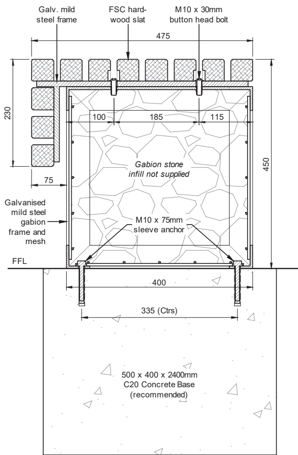
Bench base fix detail
