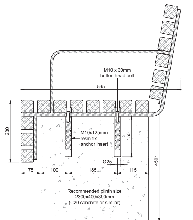
Seat base fix detail
