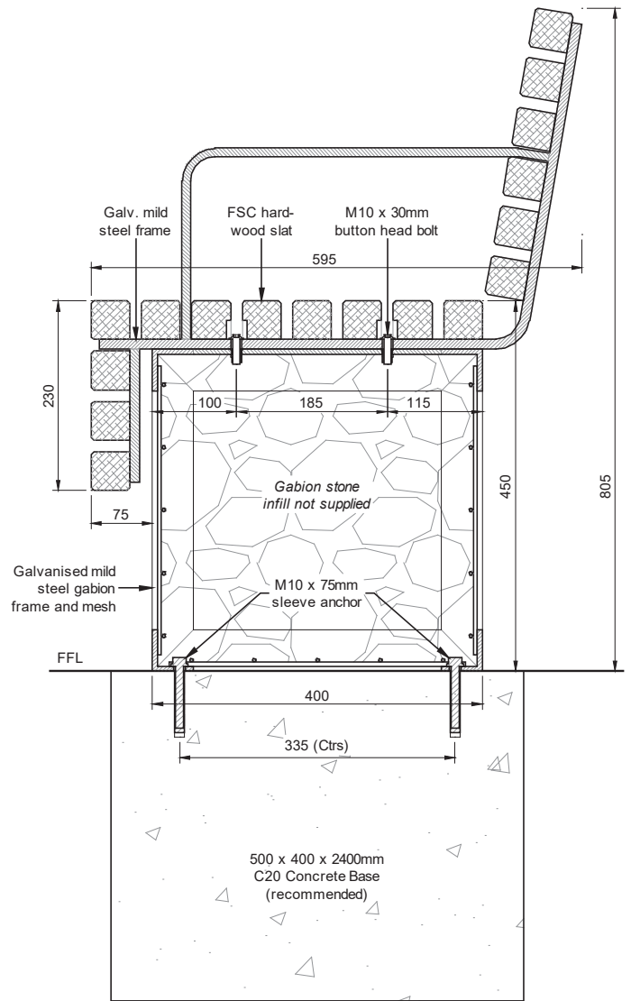
Seat base fix detail
