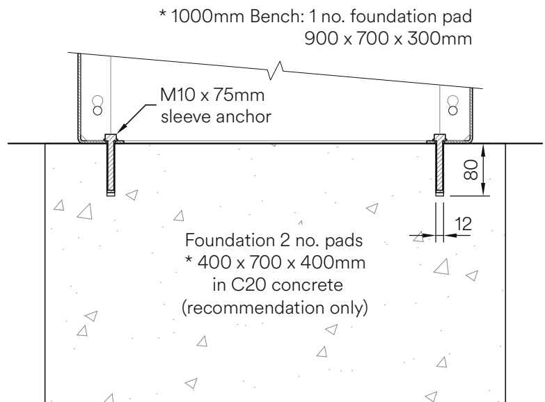
Base Fixing Detail
